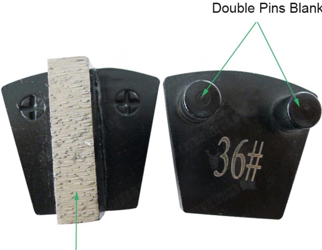
40*10*10mm*1T Single Diamond Segment
