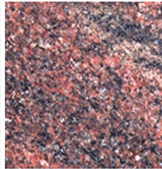
Granite
